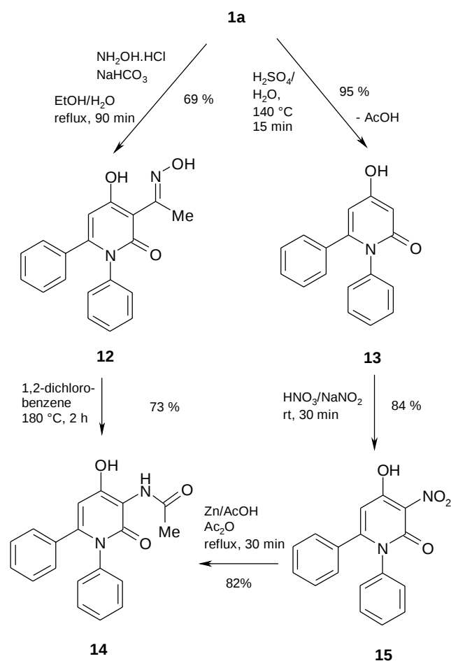
Scheme 4 Beckmann rearrangement of 3-(1-hydroxyiminoethyl)-pyridinone 12 to 3-acetylaminopyridone 14
