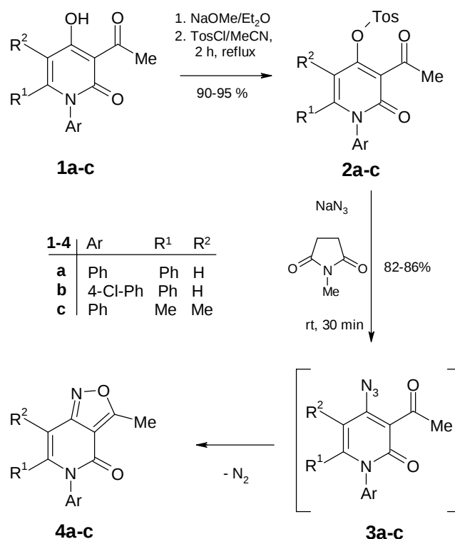
Scheme 1 Cyclization of 3-acetyl-4-tosyloxy-pyridones 2 via azides 3 to isoxazolo[4,3-c]pyridones 4
